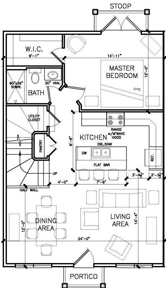
1st FLOOR PLAN PLAN 1A
